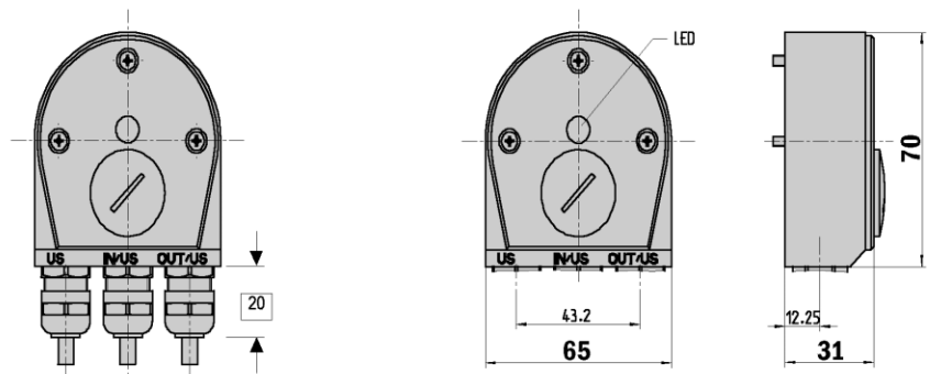
Dimensional drawing Profibus link adaptor KA3
