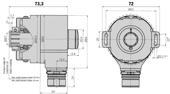
Dimensional drawing blind hollow shaft, connector radial
