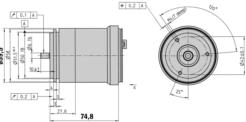
Dimensional drawing servo flange
