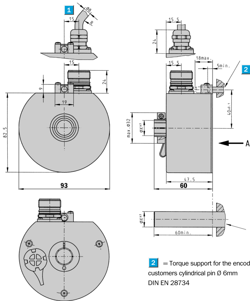
Dimensional drawing through hollow shaft; connector radial, cable radial
