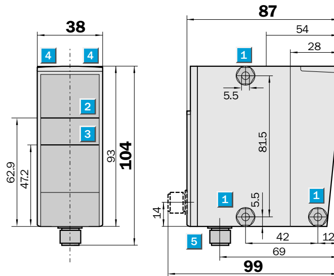
Dimensional drawing
